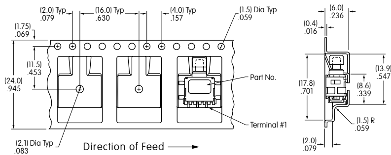
Tape Dimensions
