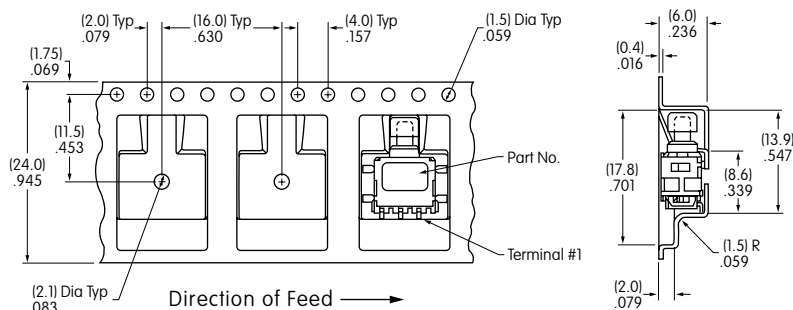
Tape Dimensions
