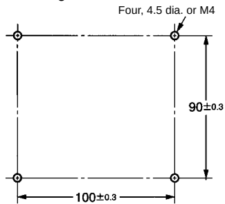
Mounting Holes
