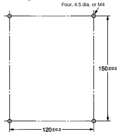
Mounting Holes
