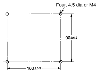
Mounting Holes
