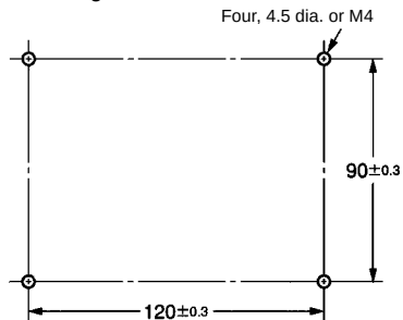
Mounting Holes
