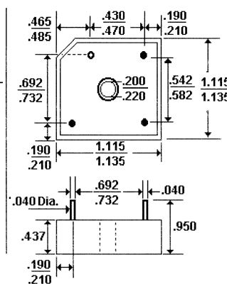
Plastic Case/Wire Leads
