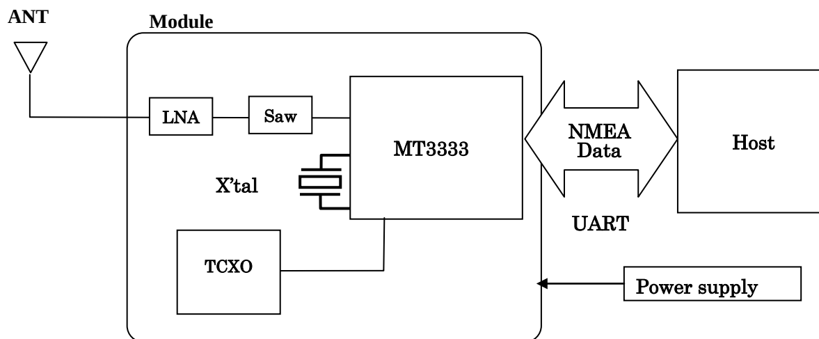
Module Block Diagram
