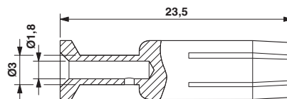
Dimensional drawing
