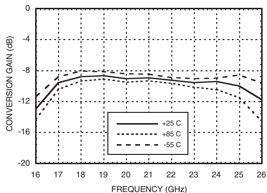
Conversion Gain vs. Temperature @ LO = -5 dBm, Vdd = +4V
