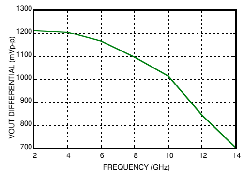
Output Differential vs. Frequency
