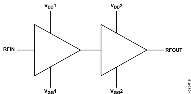
Figure 19. Basic Schematic for the HMC902
