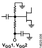
Figure 6. V GG1 , V GG2 Interface Schematic
