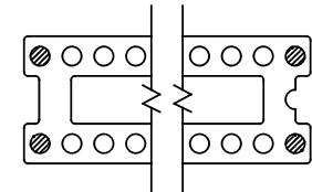
FIGURE 4 -L OPTION
