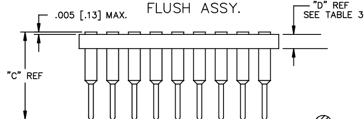
FIGURE 3 FLUSH ASSY.
