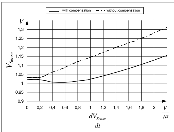
Figure 13 Overcurrent Shutdown
