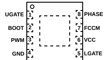
ISL6208BCRZ, ISL6208BIRZ (8 LD 2x2 DFN) TOP VIEW
