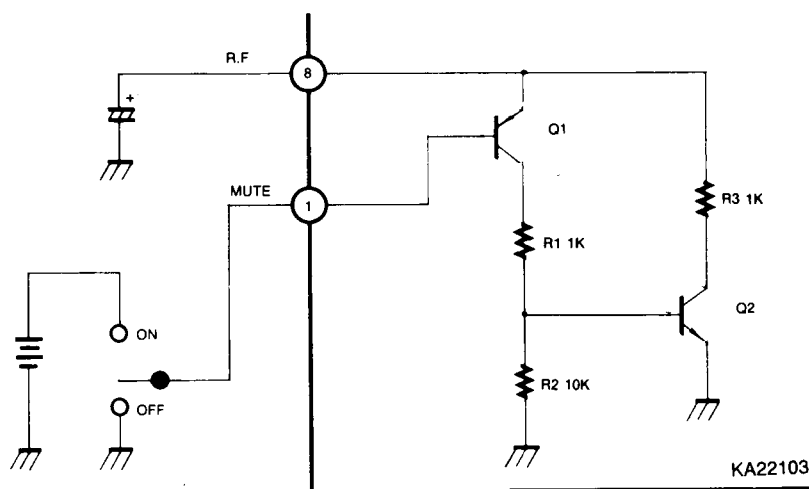
Fig. 7 MUTE Circuit
