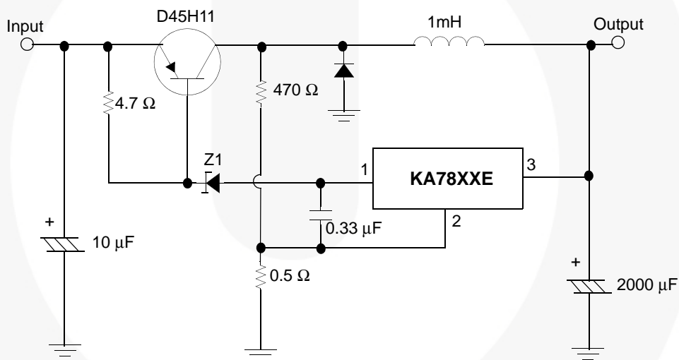
Figure 18. Switching Regulator
