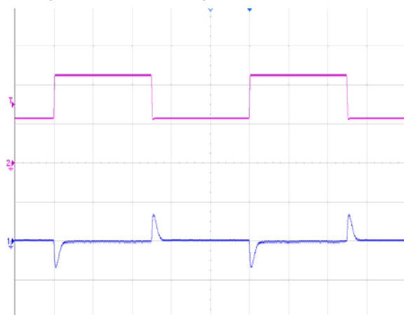
Figure 6 Dynamic response for 25% load step (25% ~ 50% ~ 75%) and 0.1A/ \mu s slew rate, see Figure 13 for test configuration, CH1-output voltage (500mV/div); CH2-output current (5A/div)
