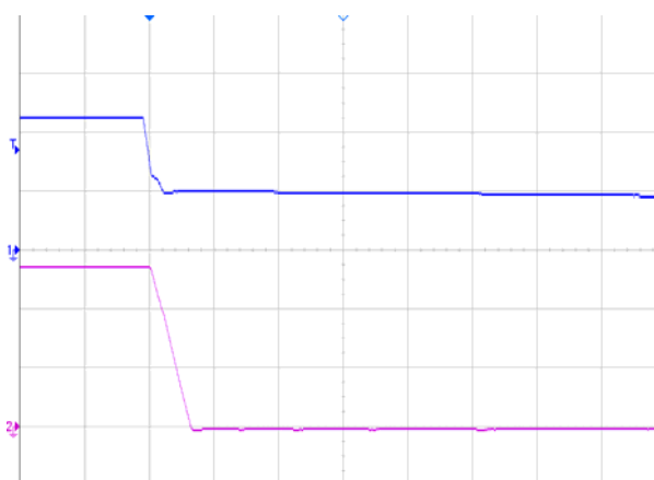
Figure 9 Output voltage shut down by power off, (2ms/div), see Figure 13 for test configuration, CH1-input voltage (10V/div); CH2-output voltage (10V/div)
