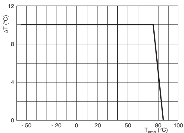
Max. allowed component temperature as a function of ambient temperature
