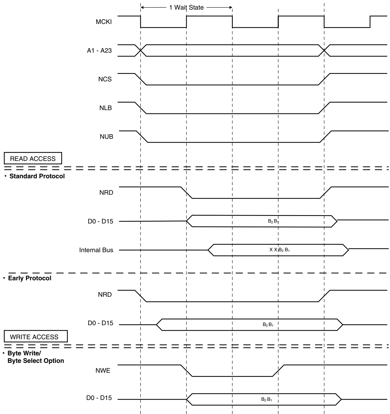
Figure 11-23. 1 Wait State, 16-bit Bus Width, Half-word Transfer
