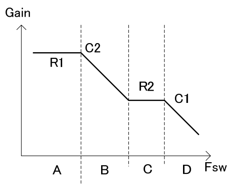
Figure 24. gm amplifier specific characteristic of frequency
