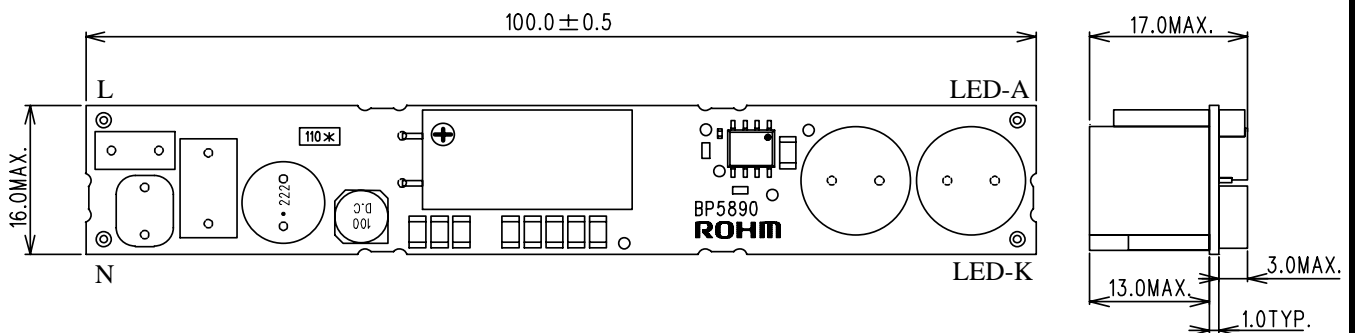
FIG.2 Dimensions
