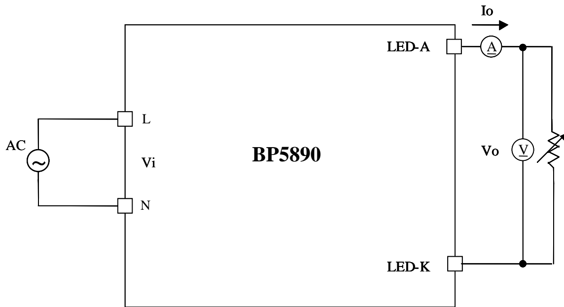
FIG.1 Test Circuit
