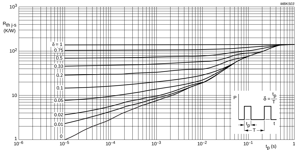
Fig.4 Transient thermal resistance from junction to soldering point as a function of pulse time; typical values.
