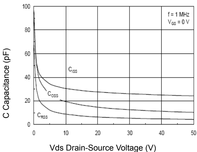
Figure 11 Capacitance vs Vds
