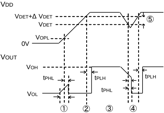
Fig.14 Timing Waveforms
