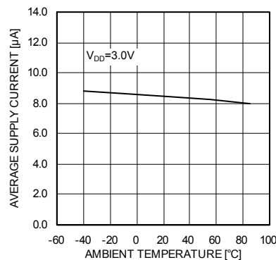
Fig.28 I_{DD} – Ambient temperature
