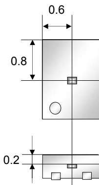
SSON004X1216
