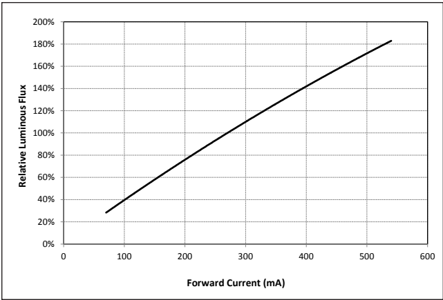
Figure 15: Vero 10D Typical Relative Luminous Flux vs. Drive Current
