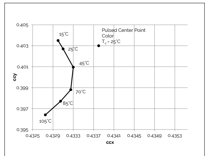
Figure 32: 3000K Color Shift vs. Case Temperature 1
