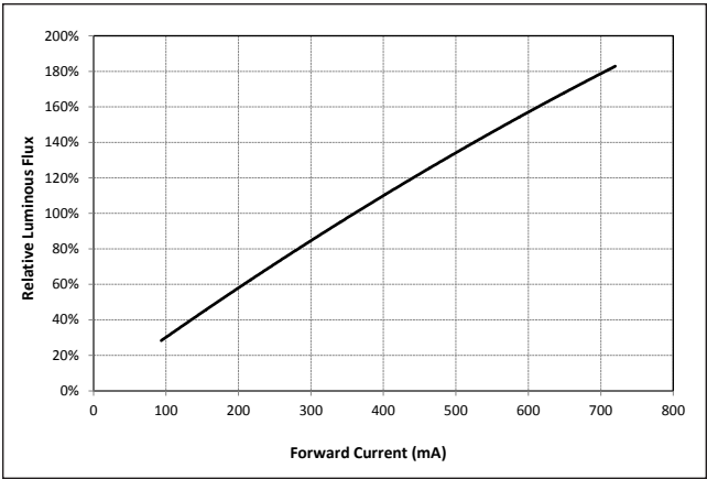
Figure 16: Vero 13B Typical Relative Luminous Flux vs. Drive Current
