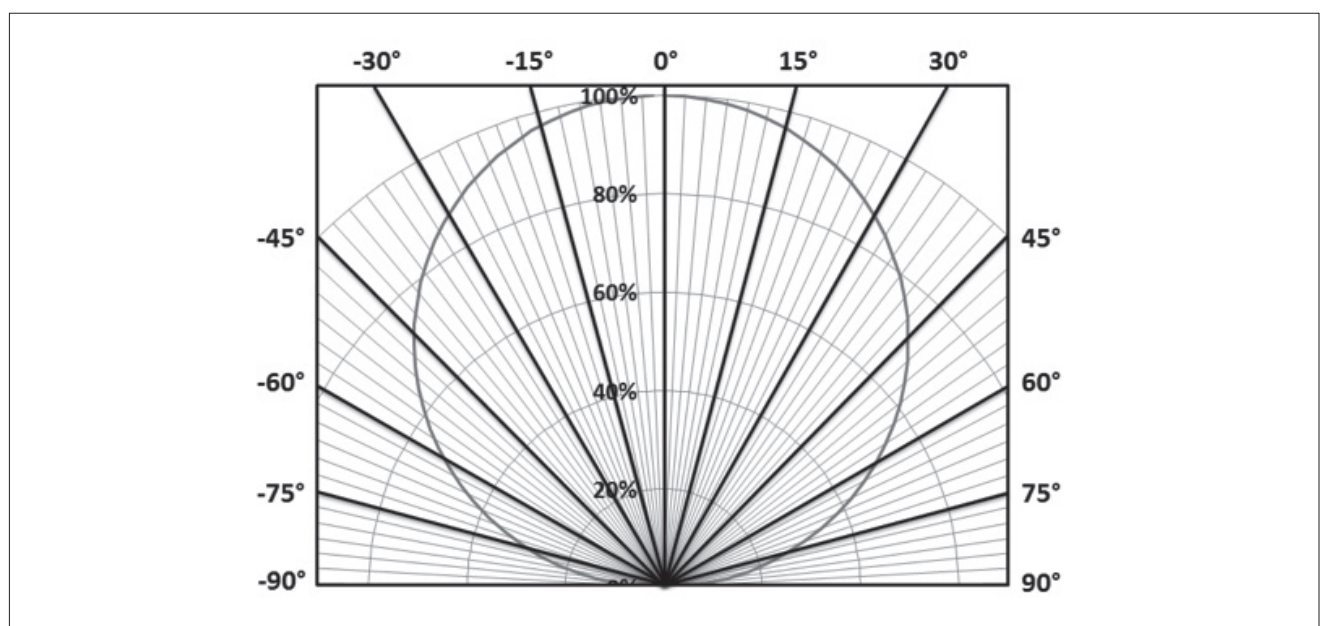
Figure 35: Typical Polar Radiation Pattern
