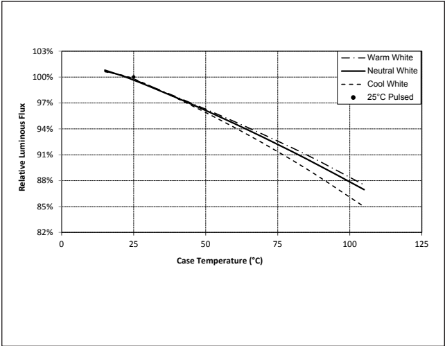
Figure 26: Vero 13 Typical DC Flux vs. Case Temperature
