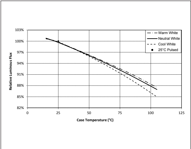
Figure 28: Vero 29 Typical DC Flux vs. Case Temperature
