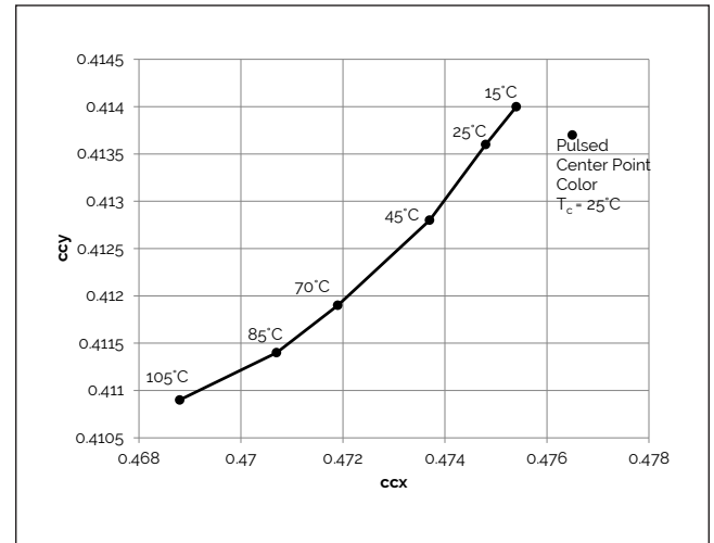
Figure 30: 2500K Color Shift vs. Case Temperature 1
