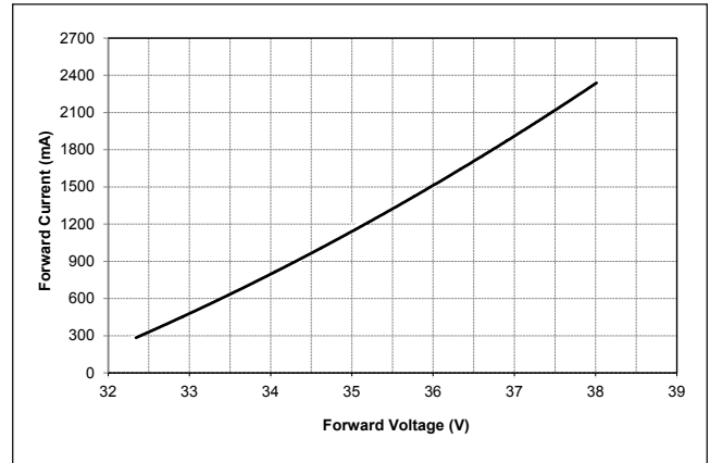
Figure 8: Vero 18C Drive Current vs. Forward Voltage ( T_j = T_c = 25^\circ\text{C} )
