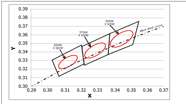
Figure 25: Graph of Cool White Test Bins in xy Color Space
