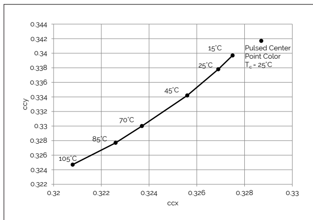
Figure 15: 5600K Color Shift vs. Case Temperature 1
