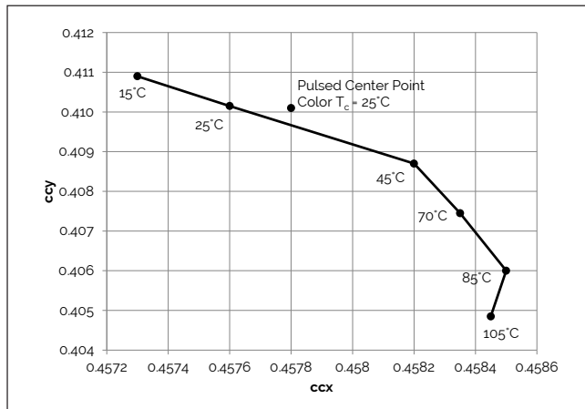
Figure 13: 2700K, 97 CRI Color Shift vs. Case Temperature 1
