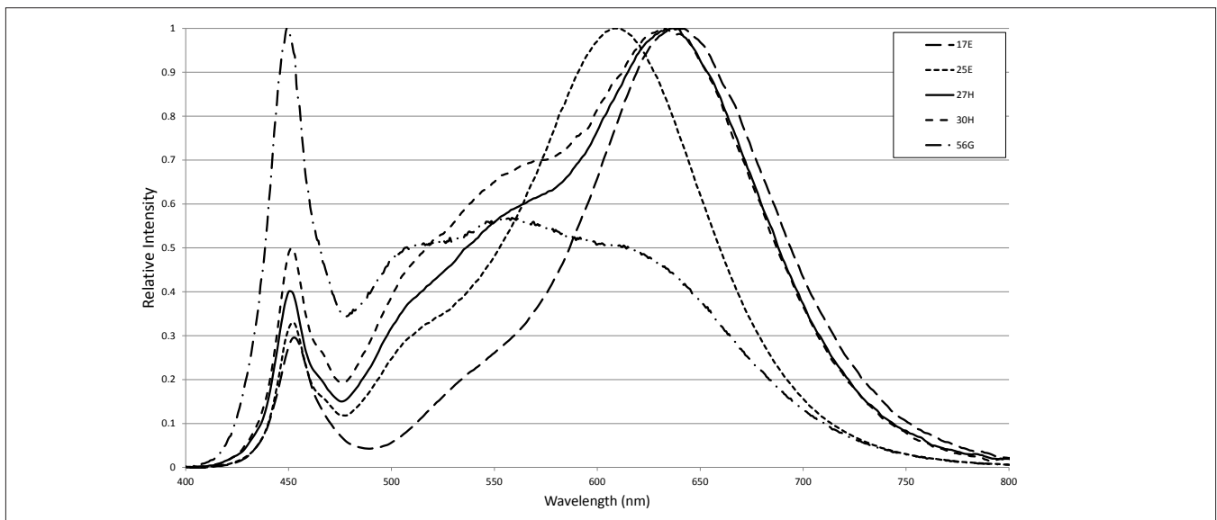
Figure 22: Typical Color Spectrum for Vero SE 18 with Décor Series
