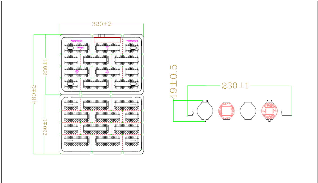
Figure 26: Drawing for Vero SE 18 Packaging Tray
