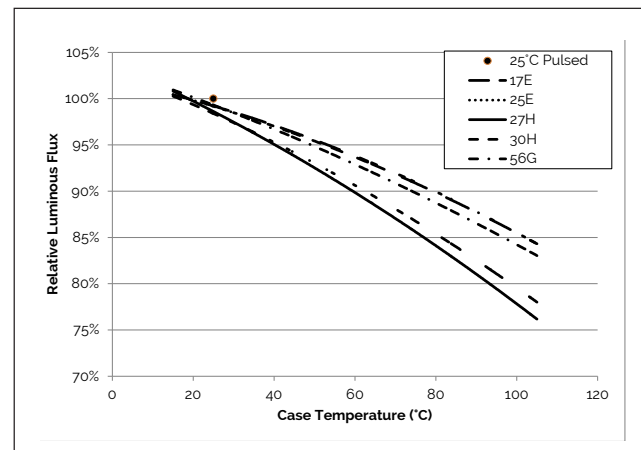
Figure 8: Décor Series Typical DC Flux vs. Case Temperature 4
