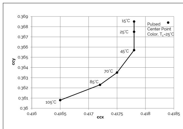
Figure 16: 3000K Class A Color Shift vs. Case Temperature 1
