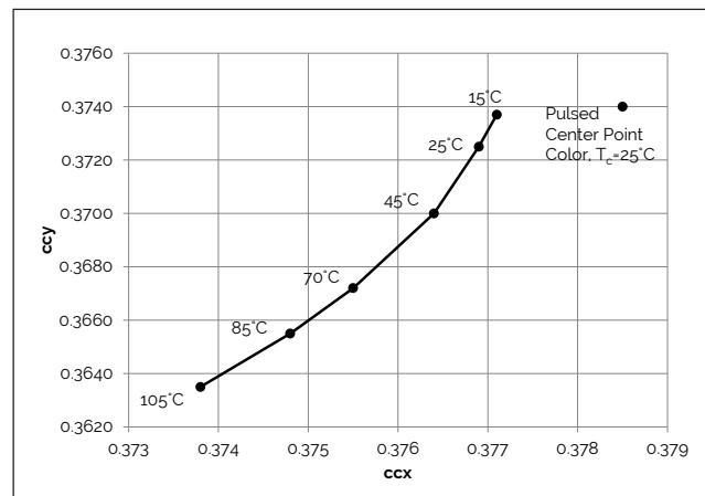
Figure 18: 4000K Class A Color Shift vs. Case Temperature 1
