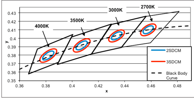
Figure 24: Graph of Warm and Neutral White Test Bins in xy Color Space
