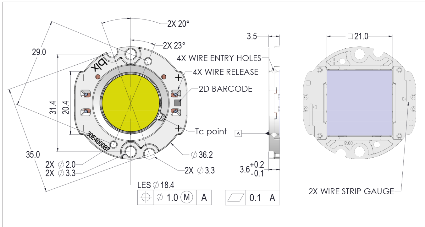
Figure 23: Drawing for Vero SE 18 LED Array
