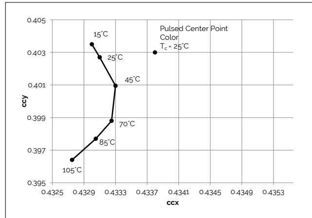
Figure 14: 3000K, 97 CRI Color Shift vs. Case Temperature 1
