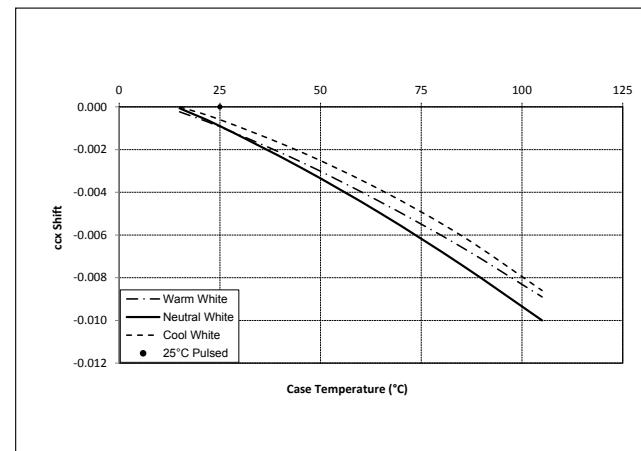
Figure 10: Typical DC ccx Shift vs. Case Temperature
