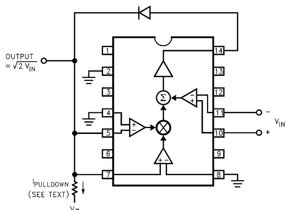
FIGURE 5. SQUARE-ROOTER
