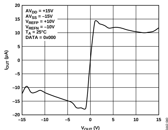
Figure 23. I_{OUT} vs. V_{OUT} ( V_{SUPPLY} = \pm 15 V )
