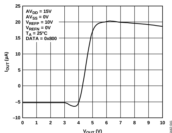
Figure 24. I_{OUT} vs. V_{OUT} ( V_{SUPPLY} = +15 V )
