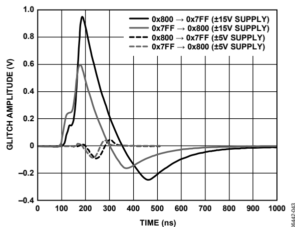
Figure 26. Output Glitch
