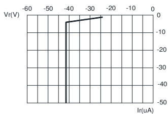
FIG.3a RED REVERSE CURRENT VS. REVERSE VOLTAGE.
