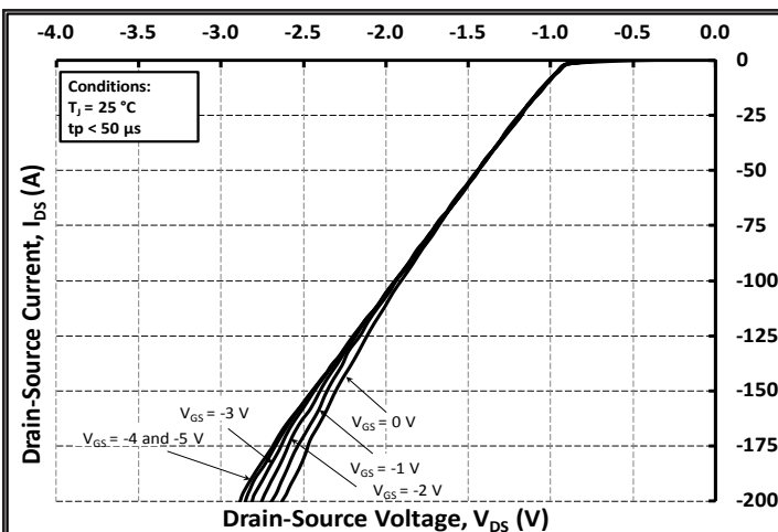
Figure 11. Typical Diode Characteristics T_J = 25^\circ\text{C}
