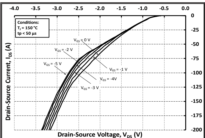
Figure 12. Typical Diode Characteristics T_J = 150^\circ\text{C}
