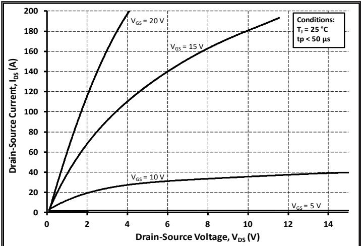
Figure 2. Typical Output Characteristics T_j = 25^\circ\text{C}
