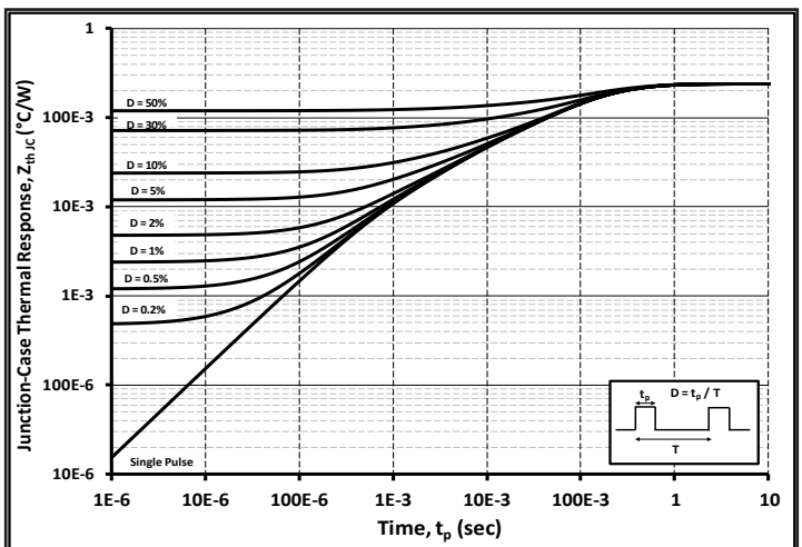
Figure 26. Transient Thermal Impedance - MOSFET
