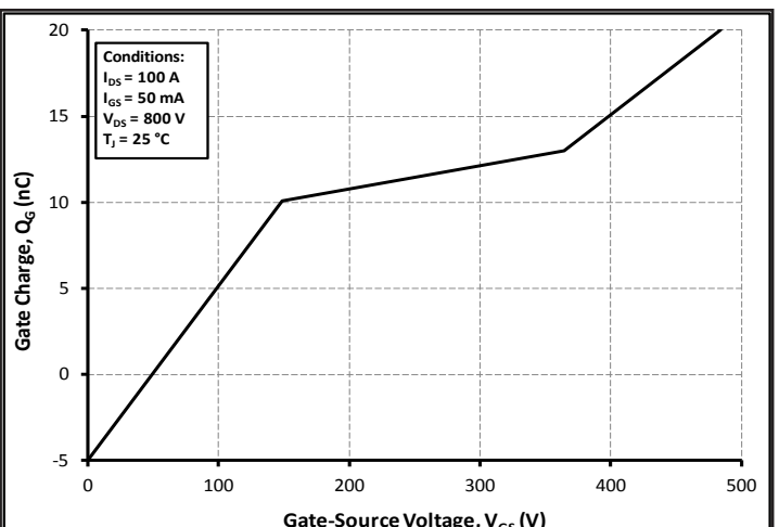
Figure 18. Typical Gate Charge Characteristic
