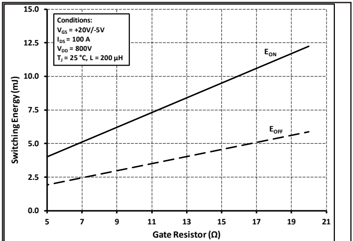
Figure 22. Clamped Inductive Switching Energy vs. Gate Resistance
