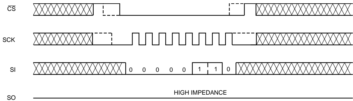
Figure 4. WREN Timing
