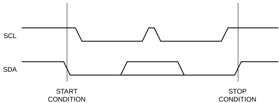
Figure 3. START/STOP Conditions
