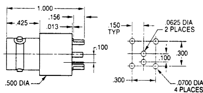
CIRCUIT BOARD JACK
