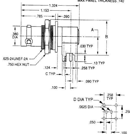
RIGHT ANGLE CIRCUIT BOARD BULKHEAD JACK
