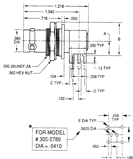
RIGHT ANGLE CIRCUIT BOARD BULKHEAD JACK
