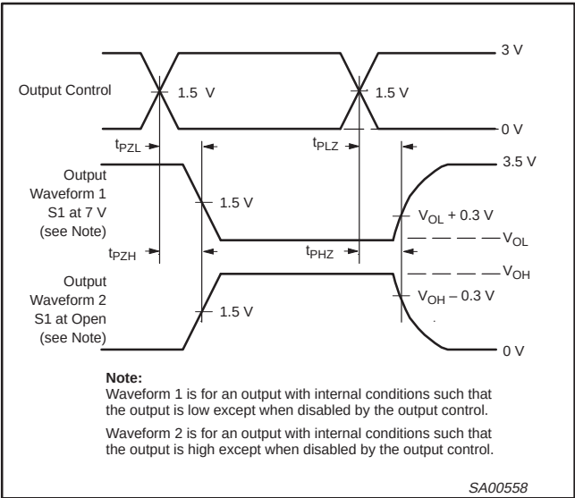
t_{PLZ} and t_{PHZ} are the same as t_{dis} . t_{PZL} and t_{PZH} are the same as t_{en} . Waveform 2. Output Enable and Disable Times
