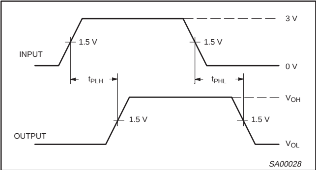
t_{PLH} and t_{PHL} are the same as t_{pd} . Waveform 1. Input to Output Propagation Delays
