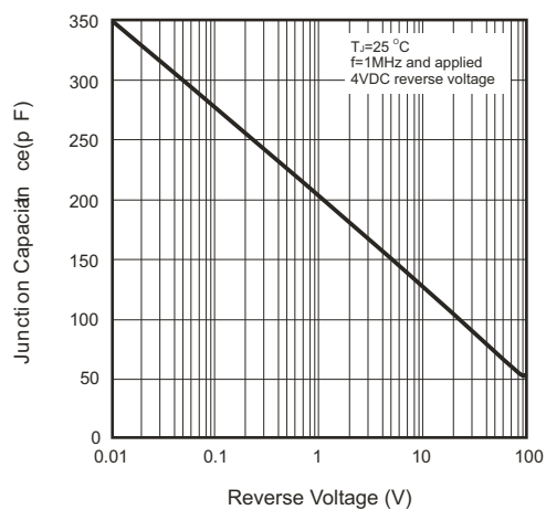
Fig.3 Junction Capacitance
