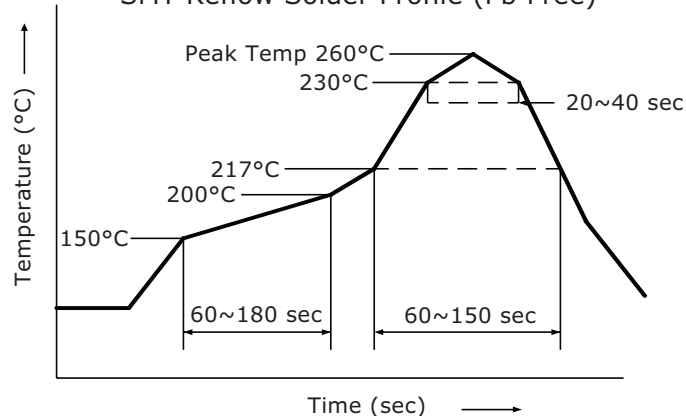
SMT Reflow Solder Profile (Pb Free)
