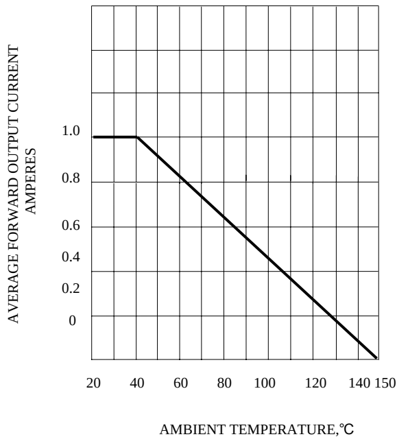
FIG. 1 - DERATING CURVE FOR OUTPUT RECTIFIED CURRENT
