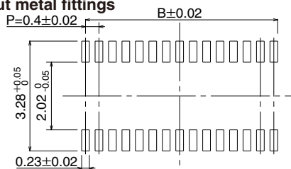
Without metal fittings
