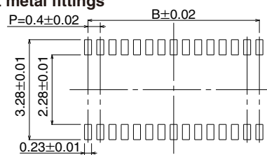
Without metal fittings
