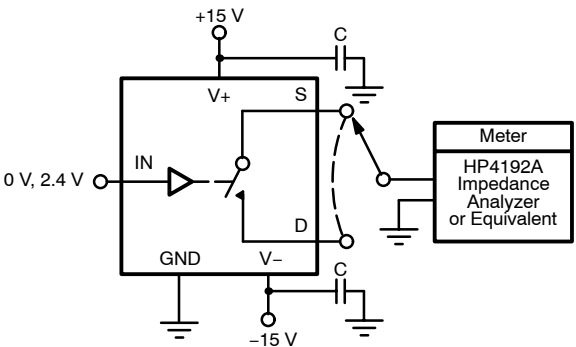
FIGURE 6. Source/Drain Capacitances
