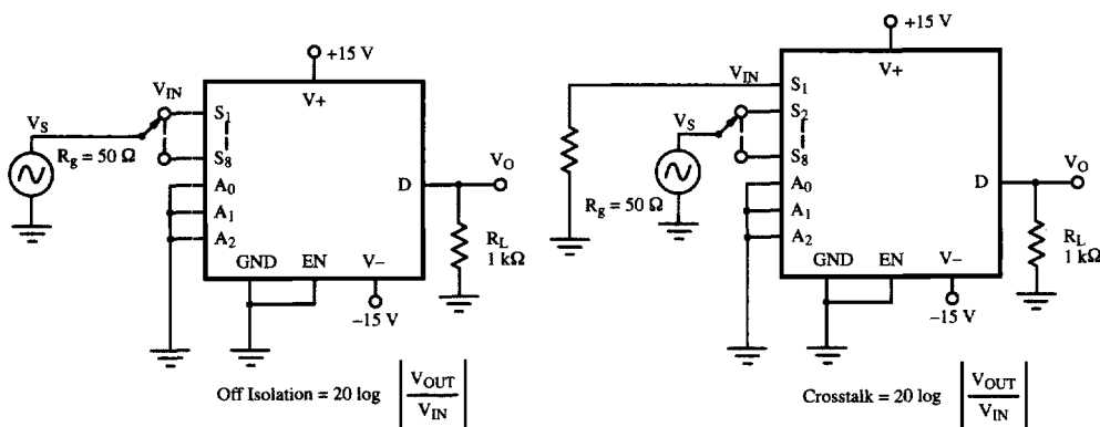
Figure 7. Crosstalk
