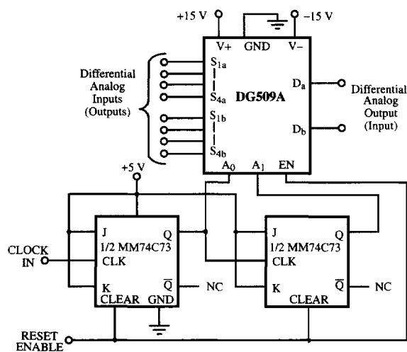
Figure 12. Differential 4-Channel Sequential Multiplexer/Demultiplexer
