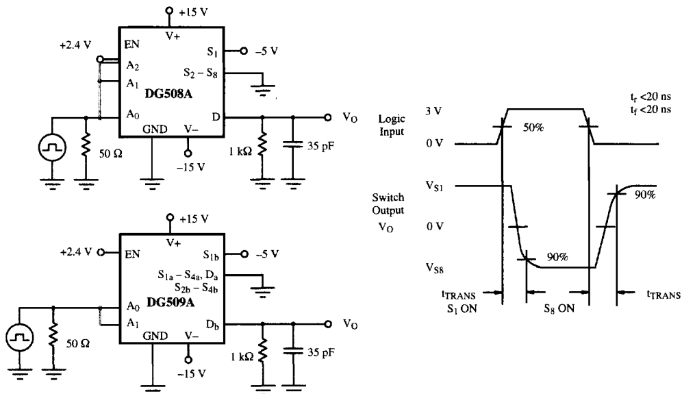
Figure 2. Transition Time
