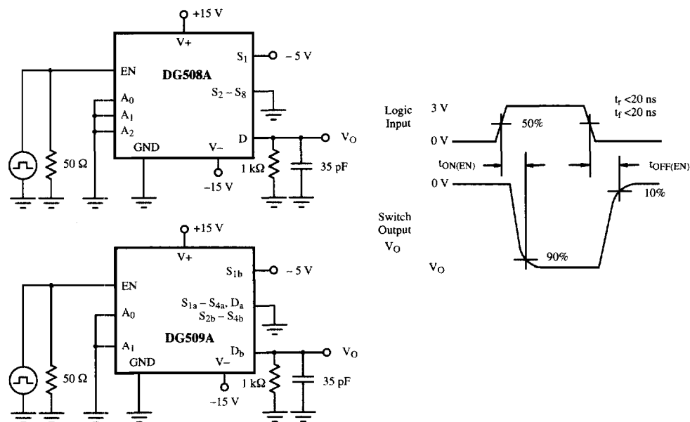
Figure 3. Enable Switching Time
