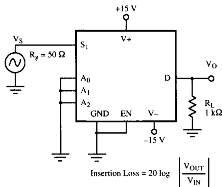
Figure 8. Insertion Loss
