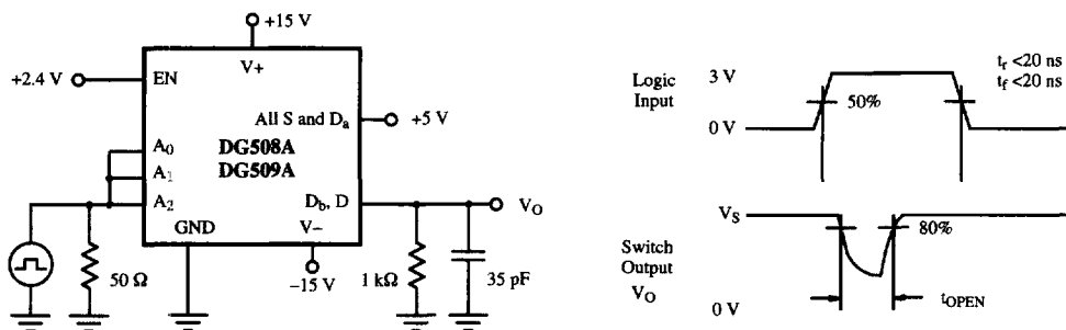
Figure 4. Break-Before-Make Interval
