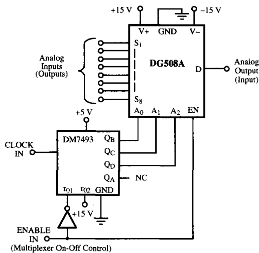
Figure 11. 8-Channel Sequential Multiplexer/Demultiplexer
