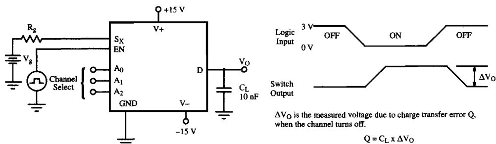
Figure 5. Charge Injection
