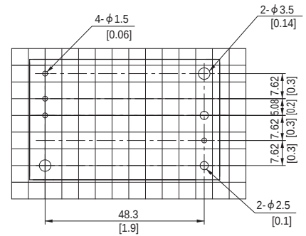
Recomending size for processing PCB (TOP VIEW)
