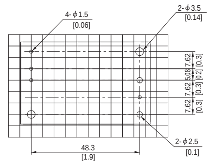
– Recomending size for processing PCB (TOP VIEW)
