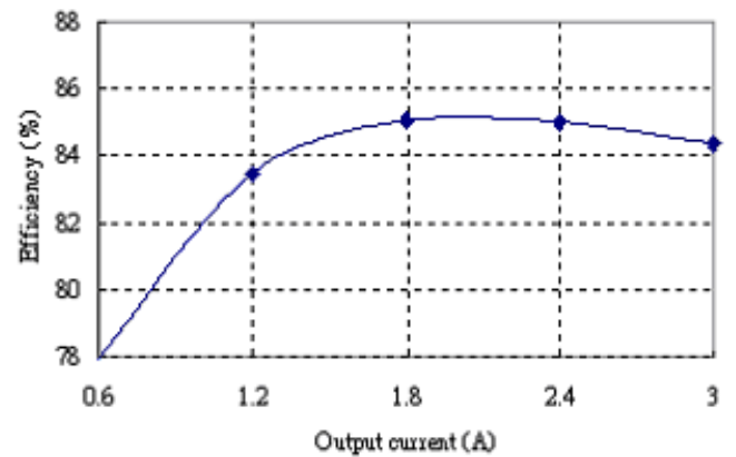
Figure 4: Converter efficiency vs. output current (12V in, 1.8V output voltage)
