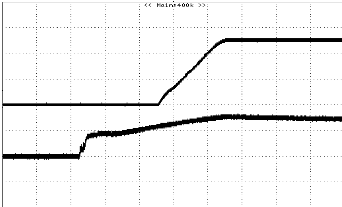
Figure 13: Turn on Using Input On/Off with external capacitors ( C_o=3000 \mu F ), 5.0V/3A out (resistive load)(2mS/div)
