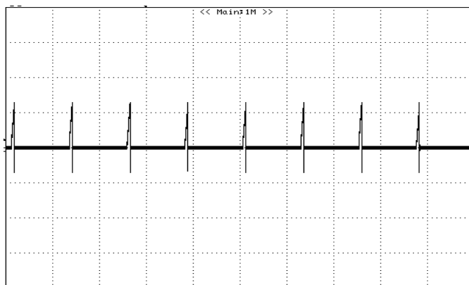
Figure 17: Output short circuit current 12Vin, 0.75Vout (0.5V/div, 50mS/div)
