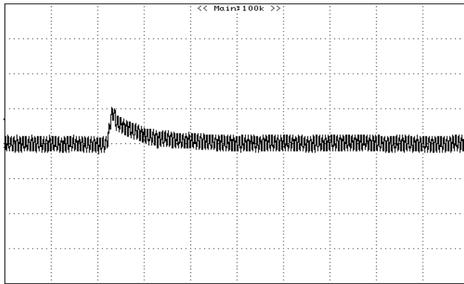
Figure 15: Typical transient response to step load change at 2.5A/\mu S from 100% to 50% of I_o , max at 12Vin, 5.0V out ( C_{out} = 1\mu F ceramic+ 47\mu F Ceramic)(100mV/div, 50uS/div)
