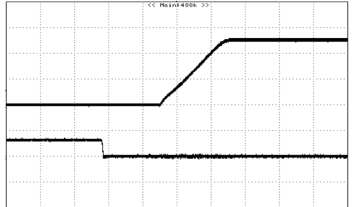
Figure 14: Turn on Using Remote On/Off with external capacitors ( C_o=3000 \mu F ), 5.0V/3A out (resistive load)(2mS/div)
