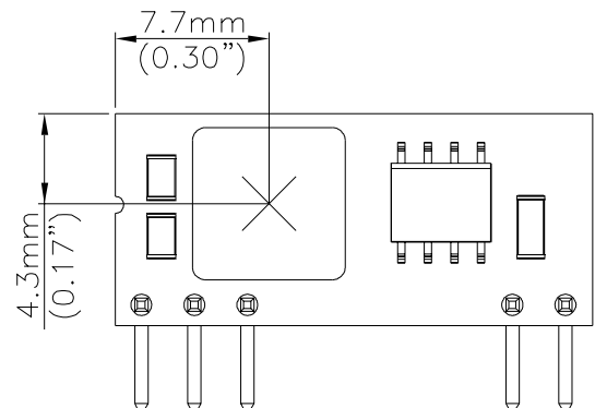
Figure 28: Temperature measurement location The allowed maximum hot spot temperature is defined at 125 °C.
