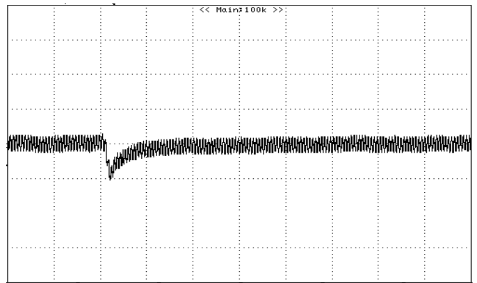
Figure 16: Typical transient response to step load change at 2.5A/\mu S from 50% to 100% of I_o , max at 12Vin, 5.0V out ( C_{out} = 1\mu F ceramic+ 47\mu F Ceramic)(100mV/div, 50uS/div)
