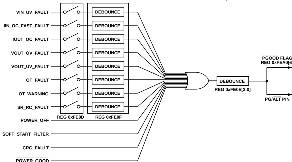
Figure 30. PGOOD Programming
