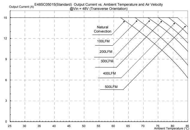
Figure 22: Output load vs. ambient temperature and air velocity @ V_{in}=48V (Transverse Orientation)
