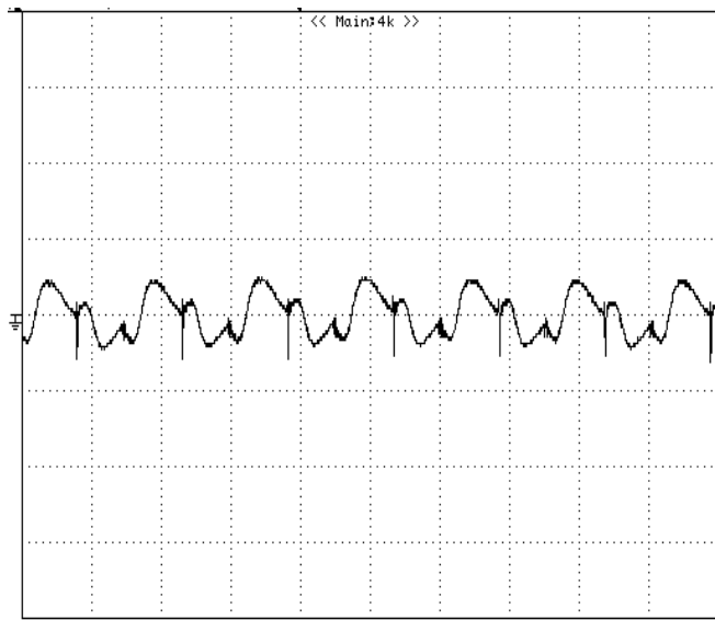
Figure 14: Output voltage ripple at nominal input voltage and rated load current ( I_o=12A ) (20 mV/div, 2us/div) Load capacitance: 1μF ceramic capacitor and 10μF tantalum capacitor. Bandwidth: 20 MHz. Scope measurements should be made using a BNC cable (length shorter than 20 inches). Position the load between 51 mm to 76 mm (2 inches to 3 inches) from the module
