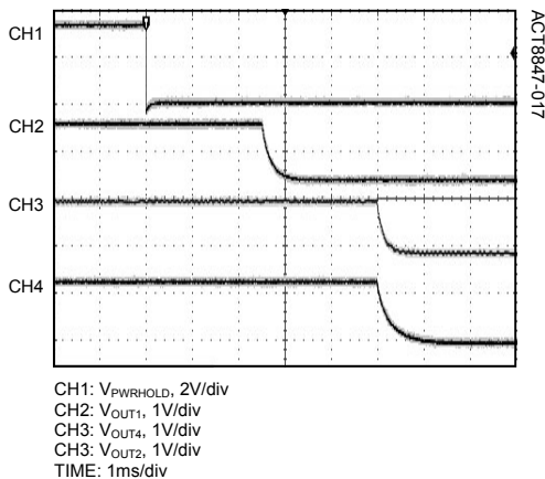
Shutdown of PWRHOLD and OUT1/4/2
