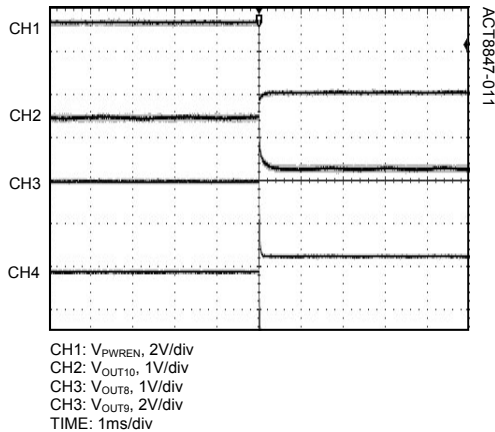
Sleep of PWREN, OUT10/8/9
