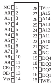
28-Pin DIP (C) (300 MIL)
