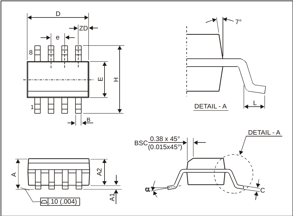
Fig. 19: SOIC8 (Small Outline Integrated Circuit)
