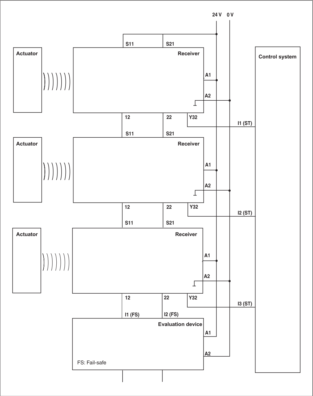
Connection diagram, series connection without SDD
