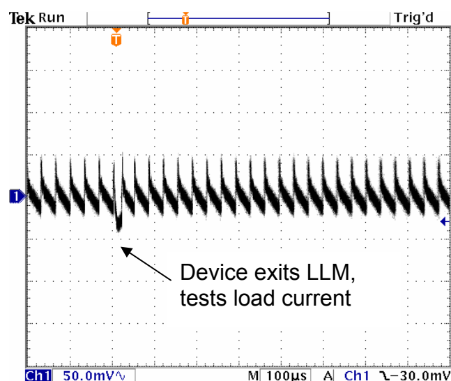
Figure 6: V_{OUT} Behavior in LLM Operation
