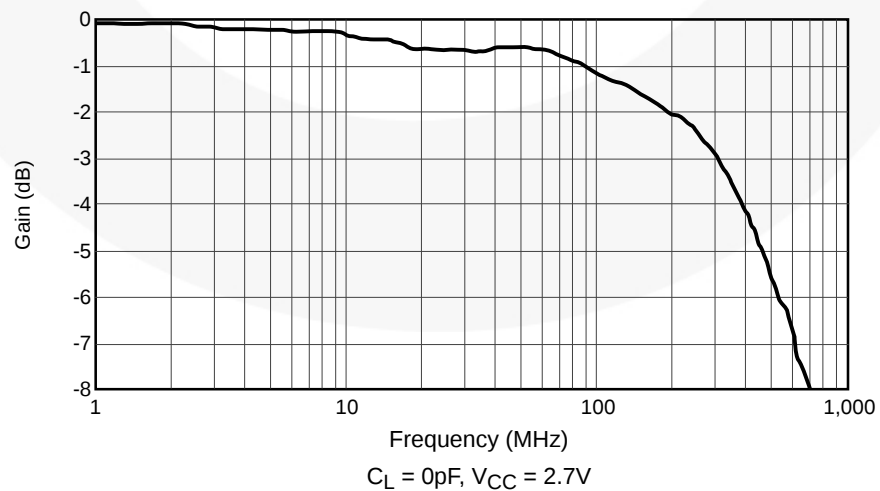
Figure 5. Bandwidth, V_{CC} = 2.7\text{ V to }5.5\text{ V}
