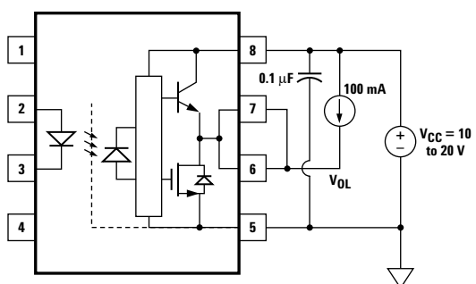
Figure 20. V_{OL} test circuit.
